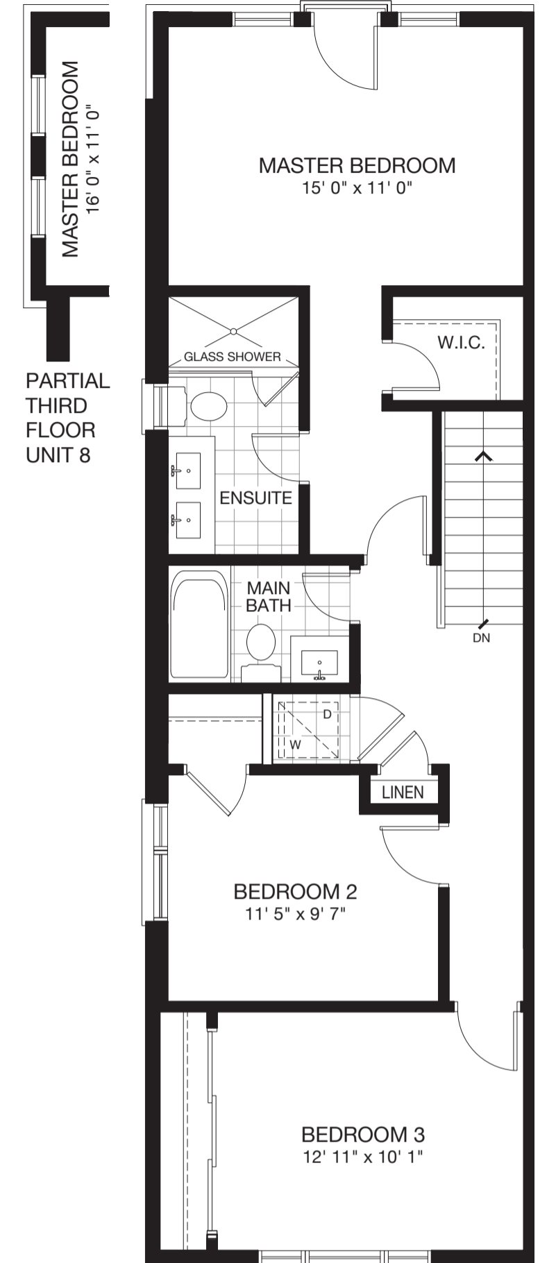
THIRD FLOOR PLAN UNIT 1
