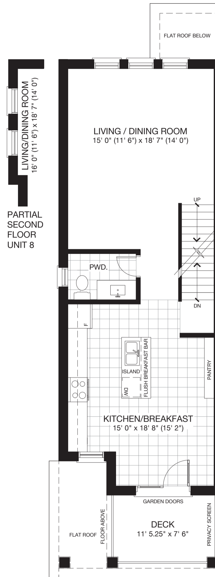
SECOND FLOOR PLAN UNIT 1
