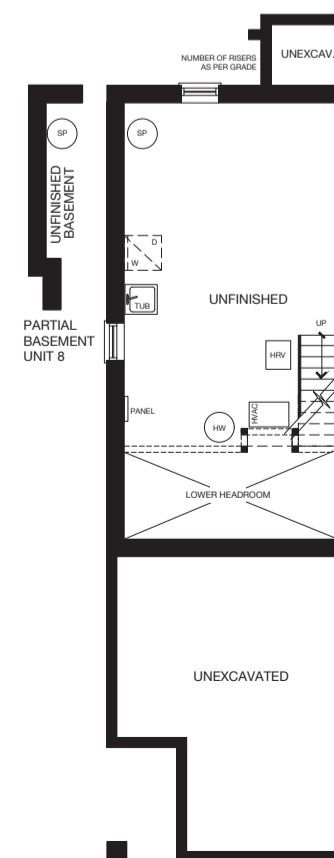
BASEMENT FLOOR PLAN UNIT 1
