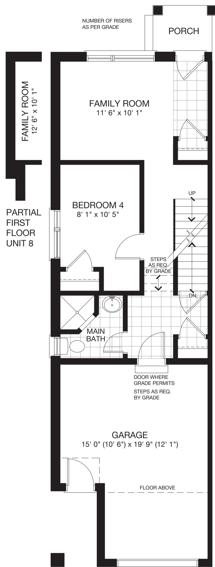
FIRST FLOOR PLAN UNIT 1
