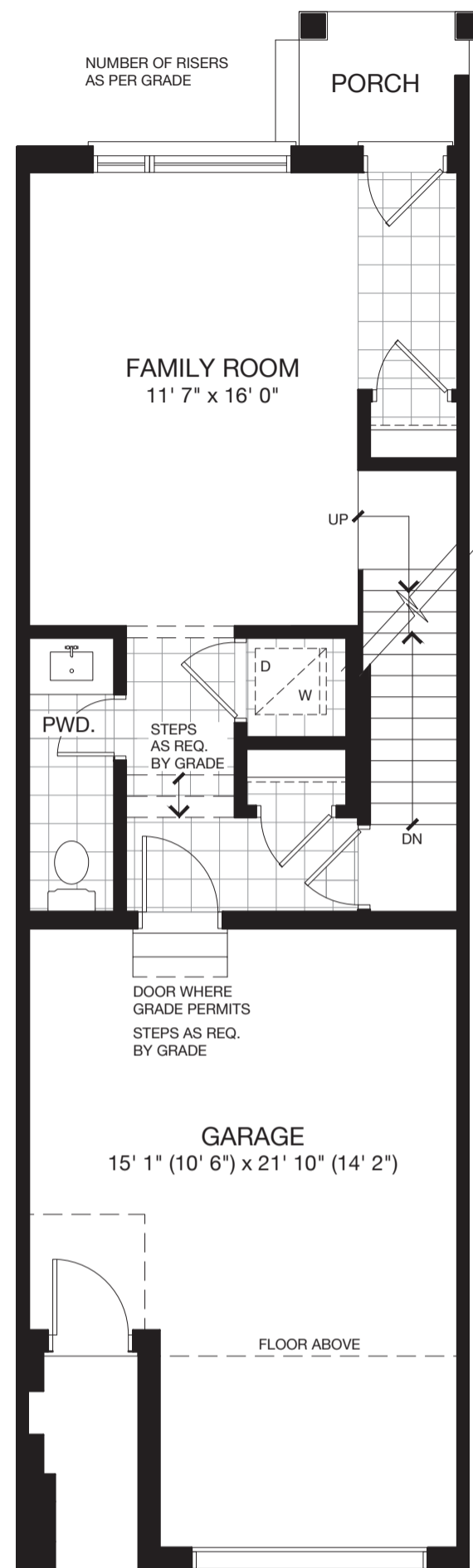
OPT. FIRST FLOOR PLAN
