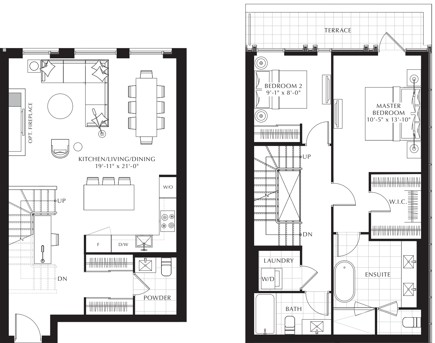
SECOND FLOOR
