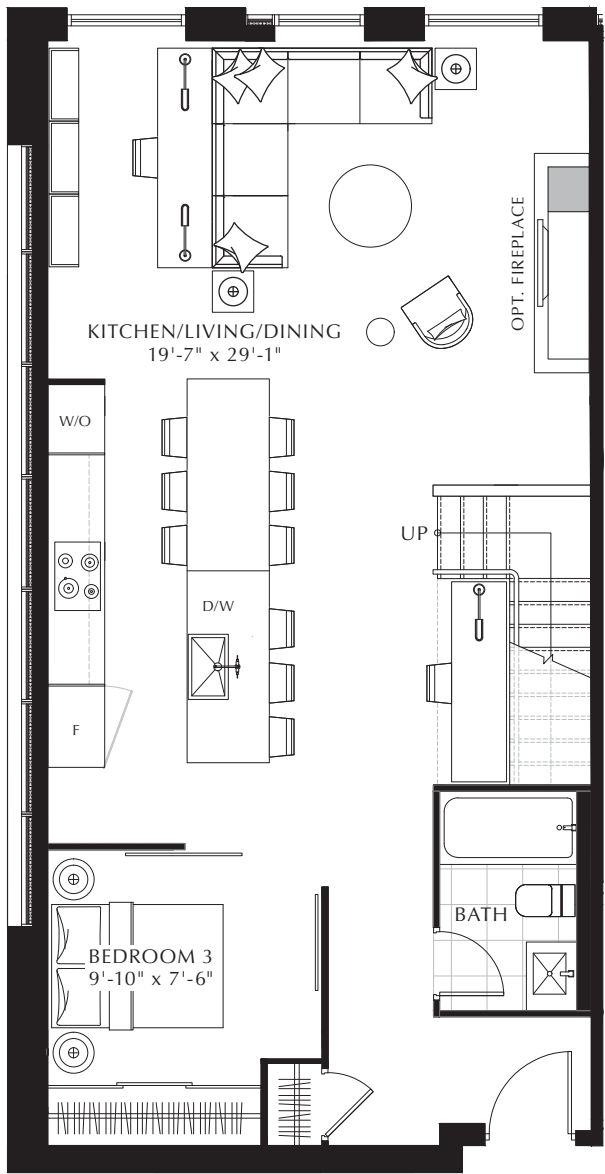
SECOND FLOOR
