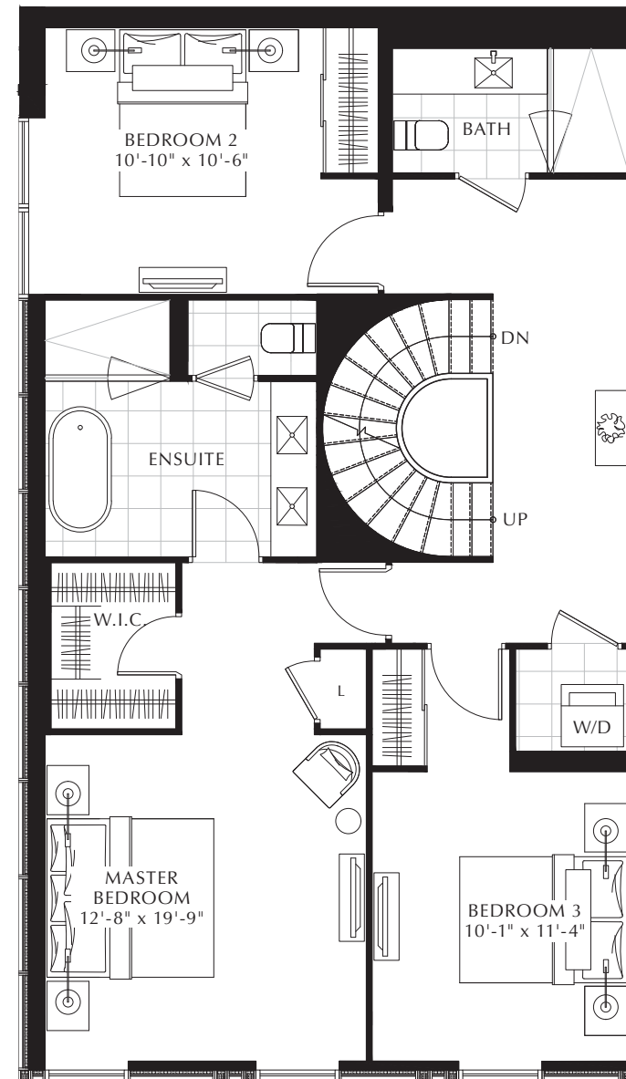
THIRD FLOOR
