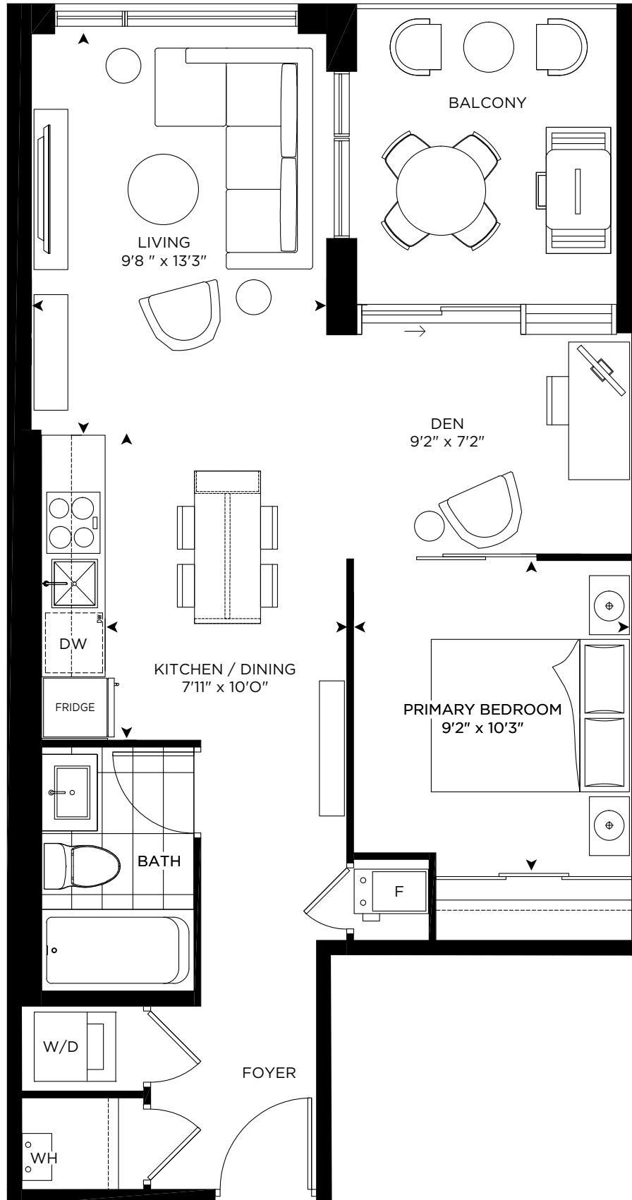
3RD FLOOR
