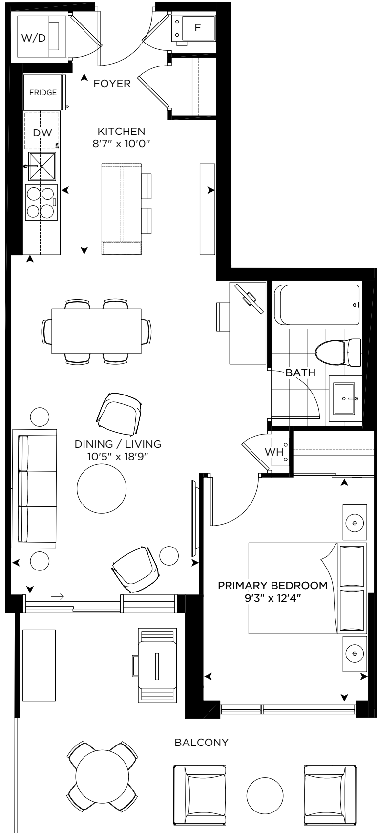
3RD FLOOR
