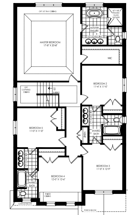
Optional 5 Bedroom Layout Elevation A
