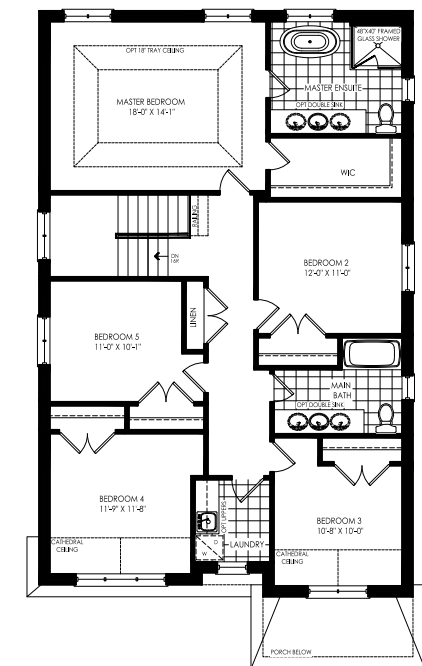
Optional 5 Bedroom Layout Elevation A
