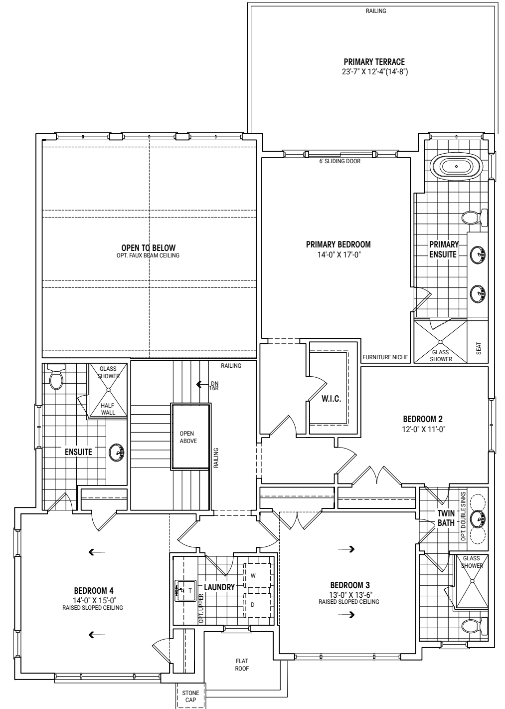
SECOND FLOOR PLAN ELEVATION B
