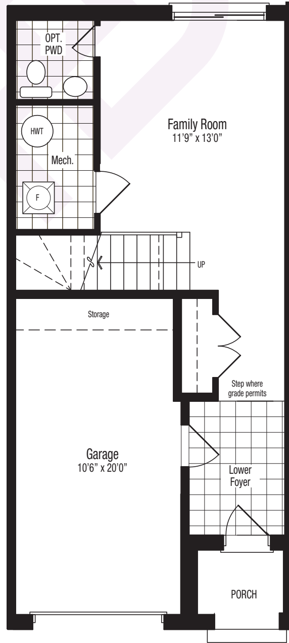
LOWER FLOOR
