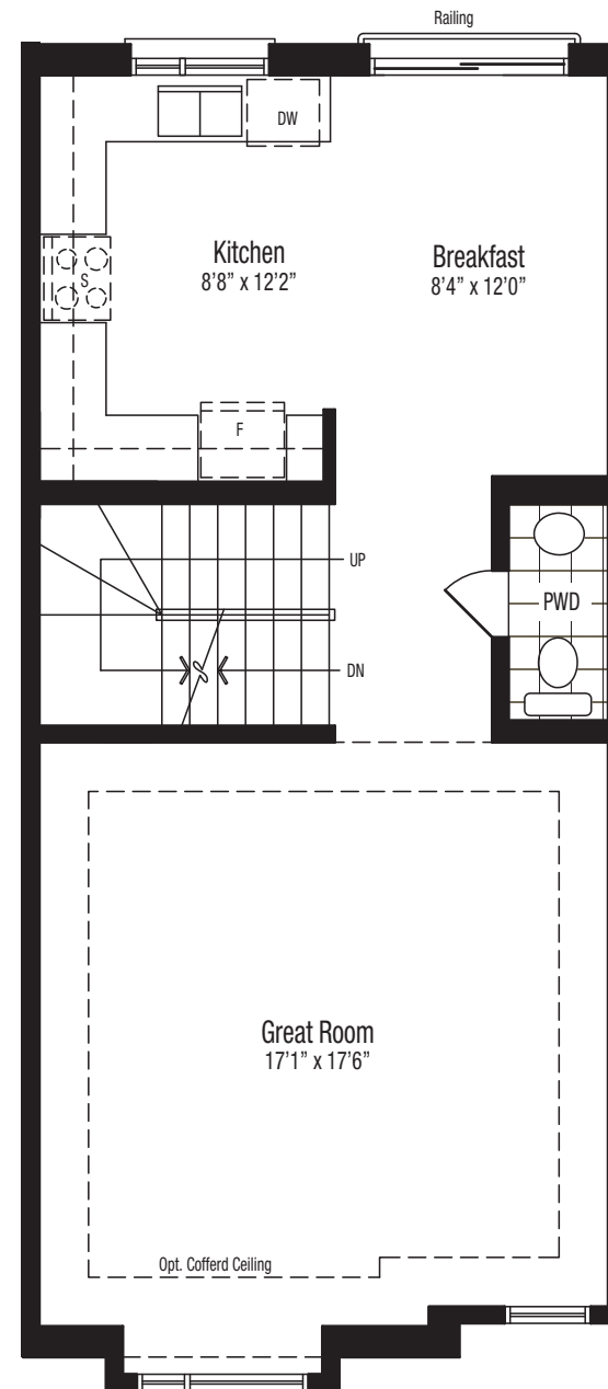
MAIN FLOOR
