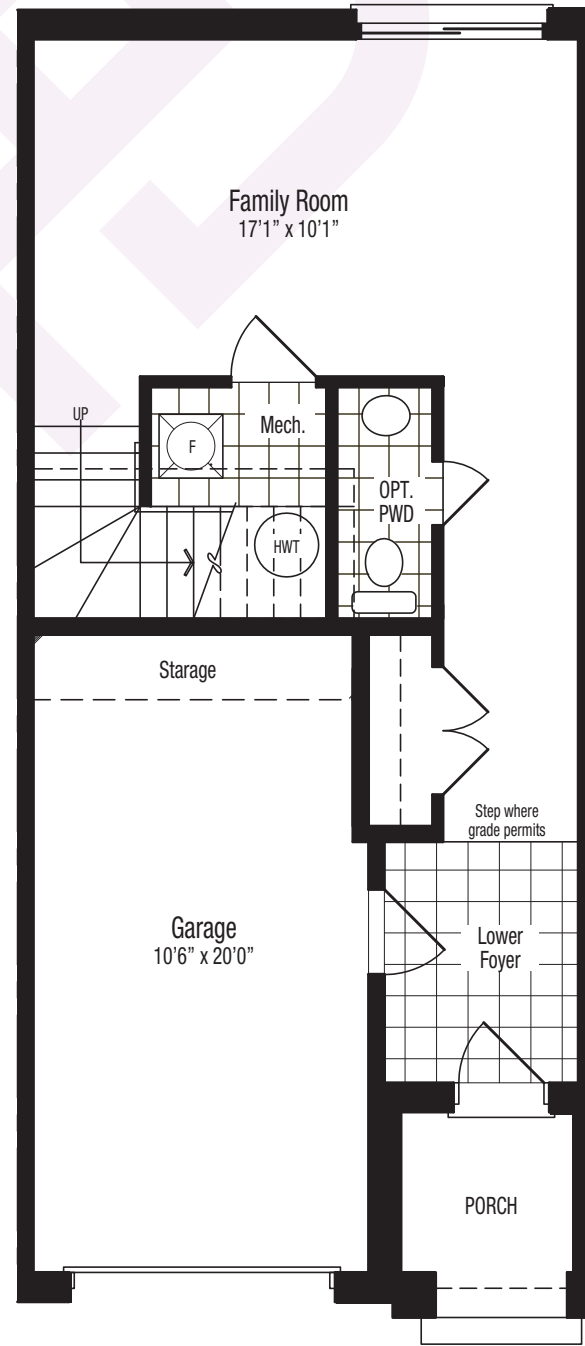
LOWER FLOOR
