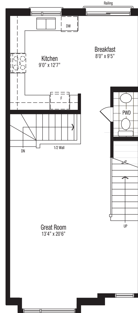
MAIN FLOOR
