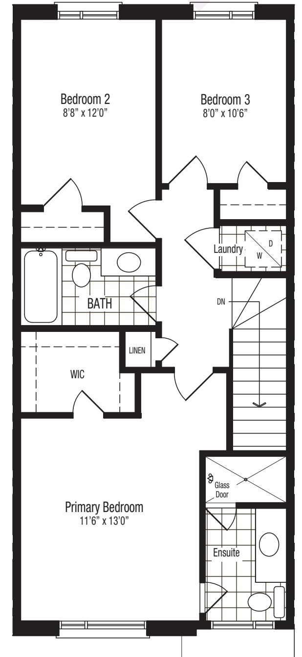
UPPER FLOOR
