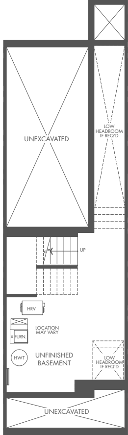
BASEMENT B
