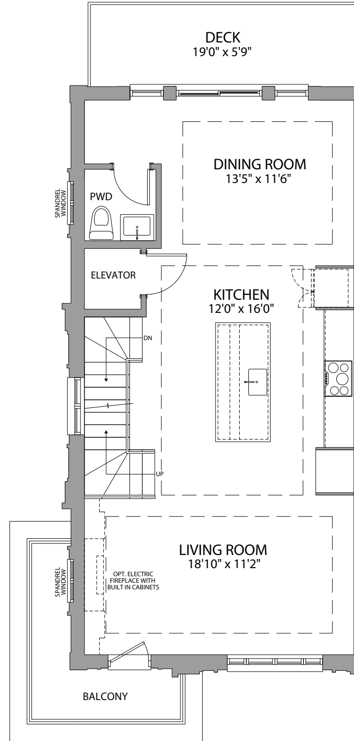
MAIN FLOOR ELEVATION A
