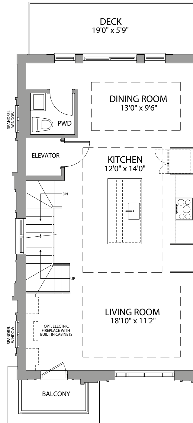
MAIN FLOOR ELEVATION A
