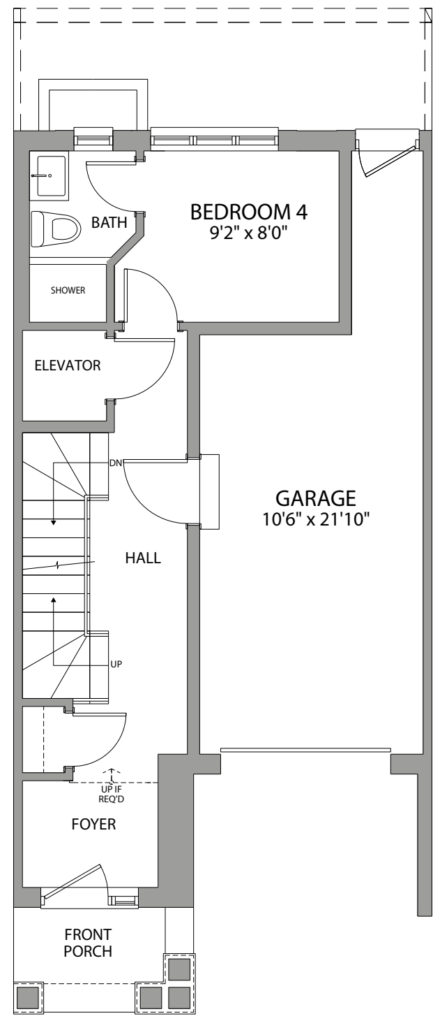
GROUND FLOOR ELEVATION A
