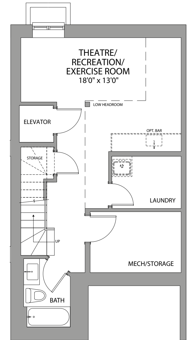
LOWER FLOOR ELEVATION A
