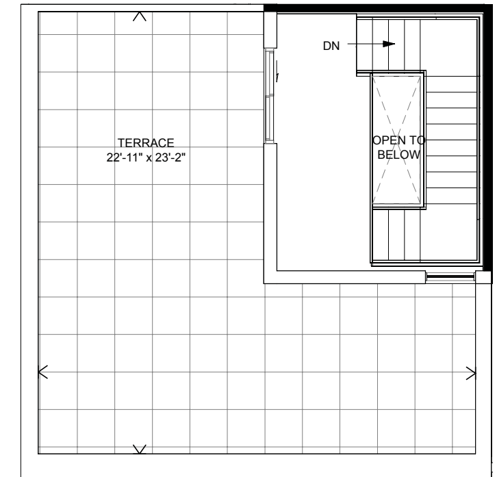
ROOF TOP TERRACE
